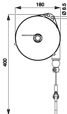
Carter aluminium
