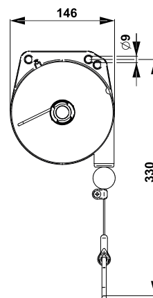
Carter aluminium
