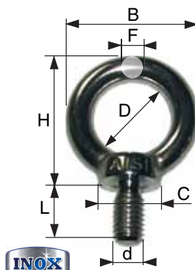
ACIER INOX
