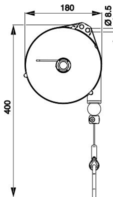
Carter aluminium
